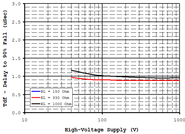
Figure 7: Fall Time Delay for different Resistive Loads at V dd = 18V
