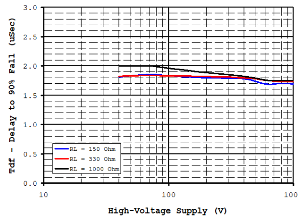
Figure 9: Fall Time Delay for different Resistive Loads at V dd = 6V
